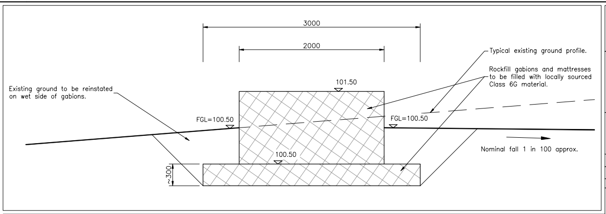
SECTION A-A TYPICAL SECTION THROUGH NEW WEIR SCALE 1:25
