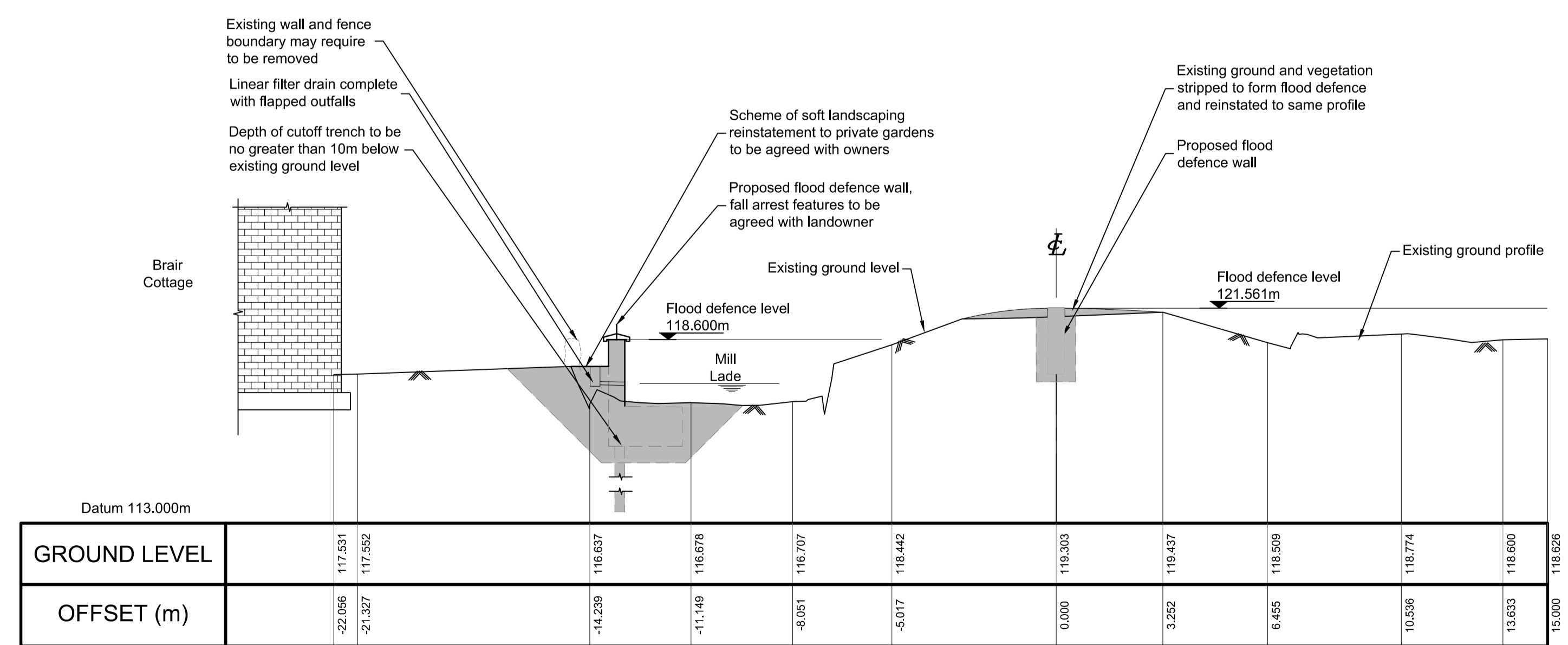
SECTION 13-EWP
