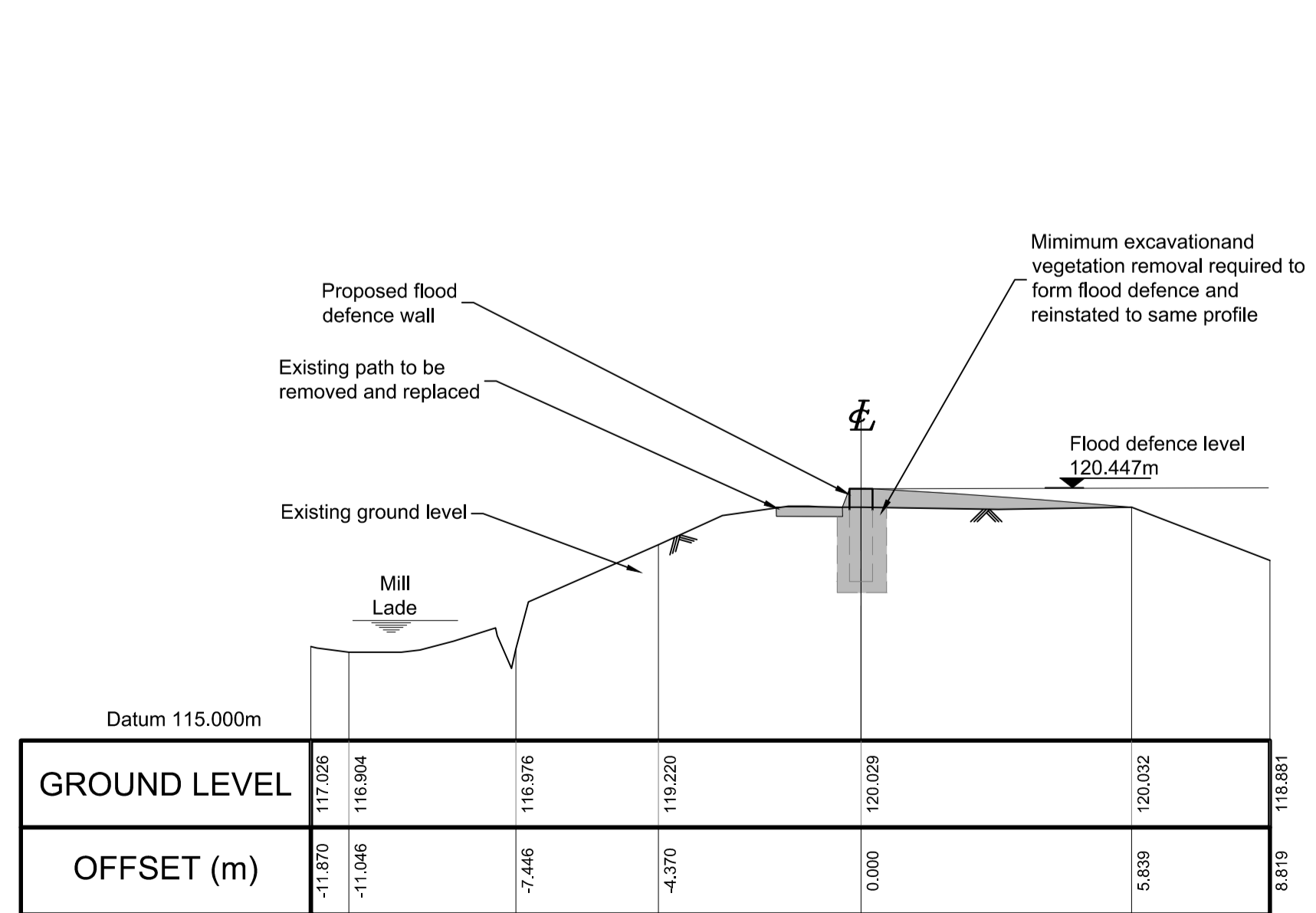
SECTION 12-EWP
